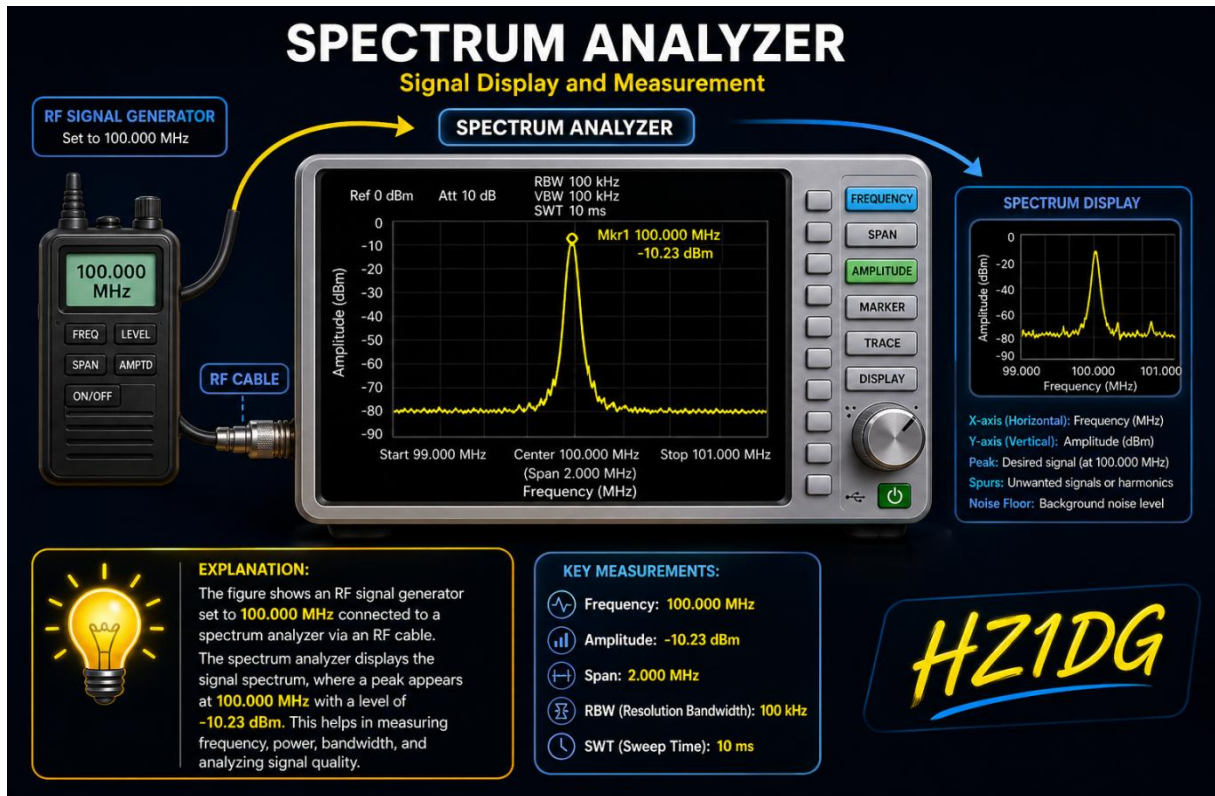
Figure (6-14): Signal display using a Spectrum Analyzer
