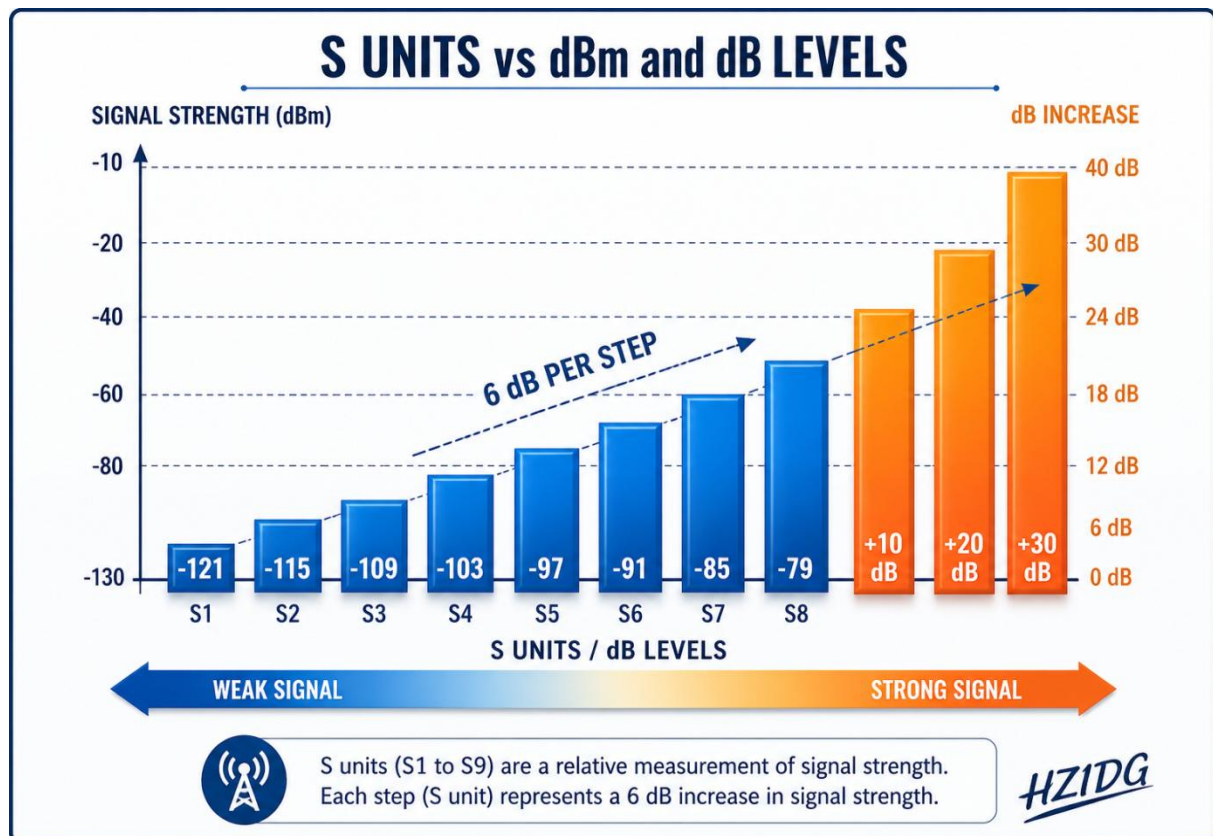
Figure (7-10): Graph of Signal Strength Above S9 (S-Meter +dB)
