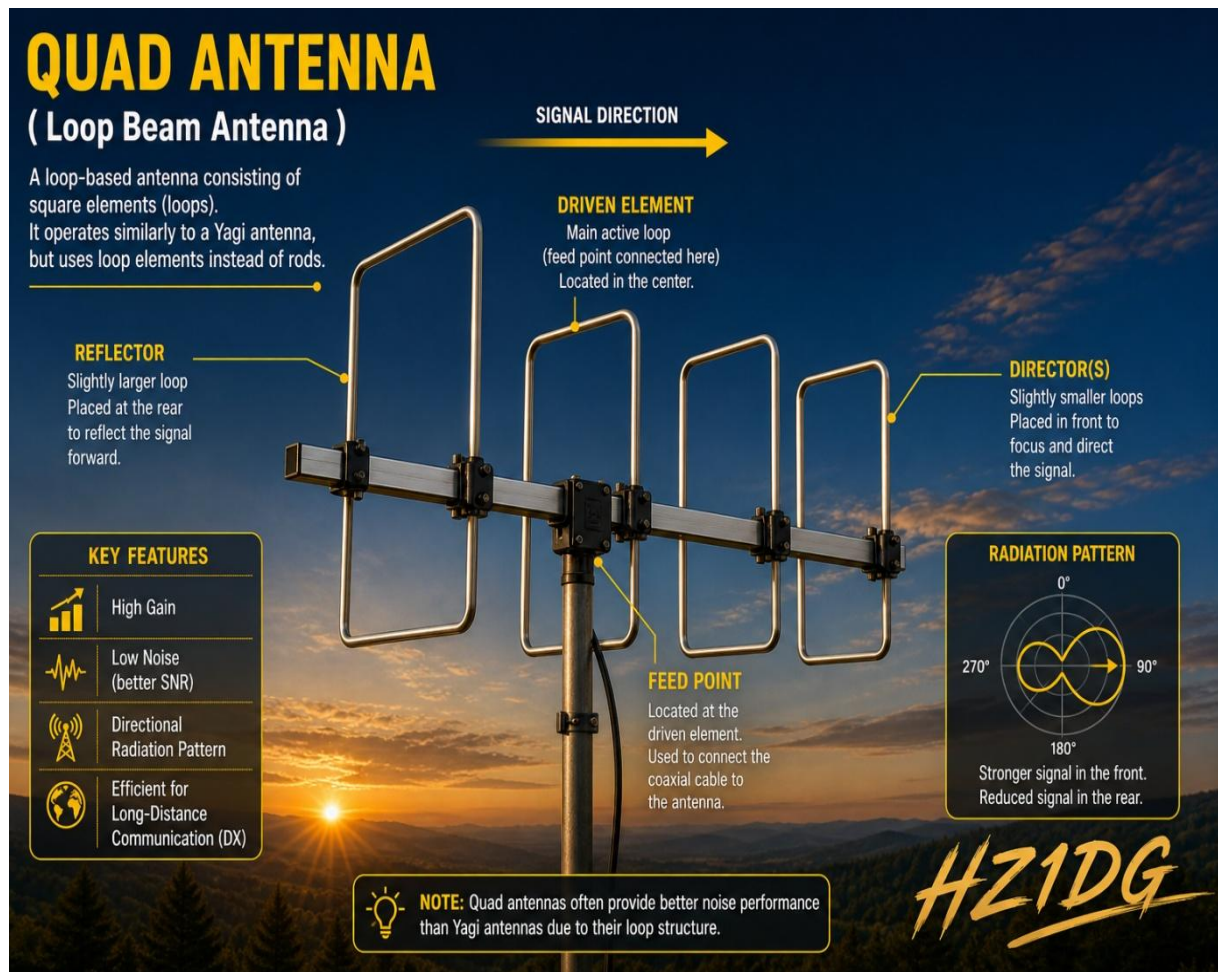
Figure (8-8): Quad antenna
