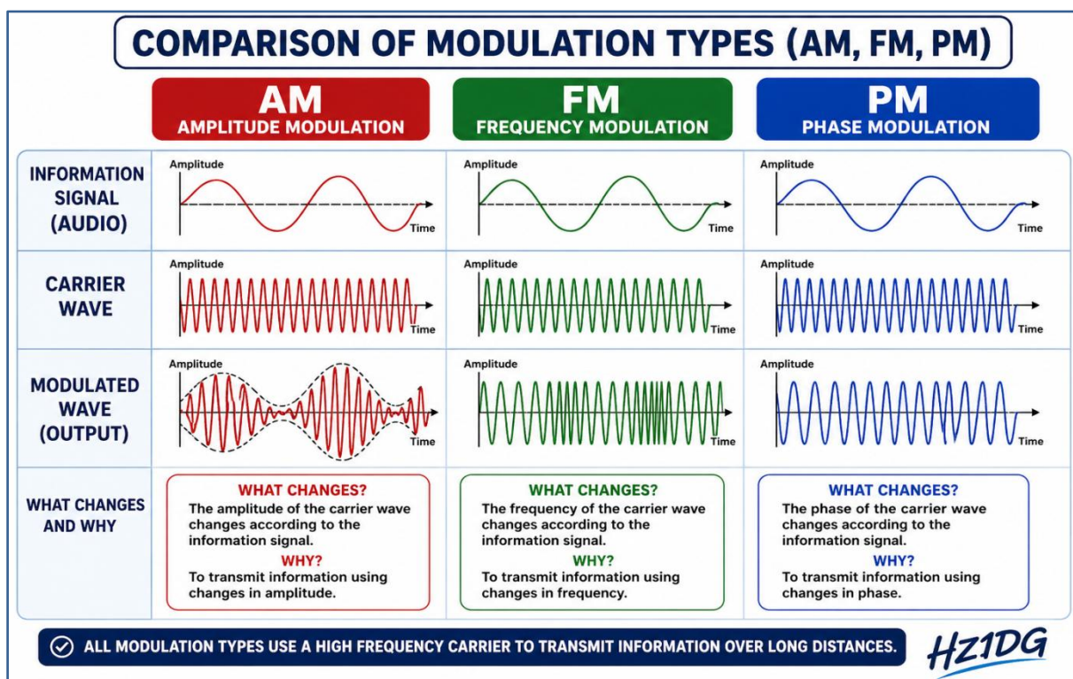
Figure (7-5): Comparison of AM, FM, and PM
