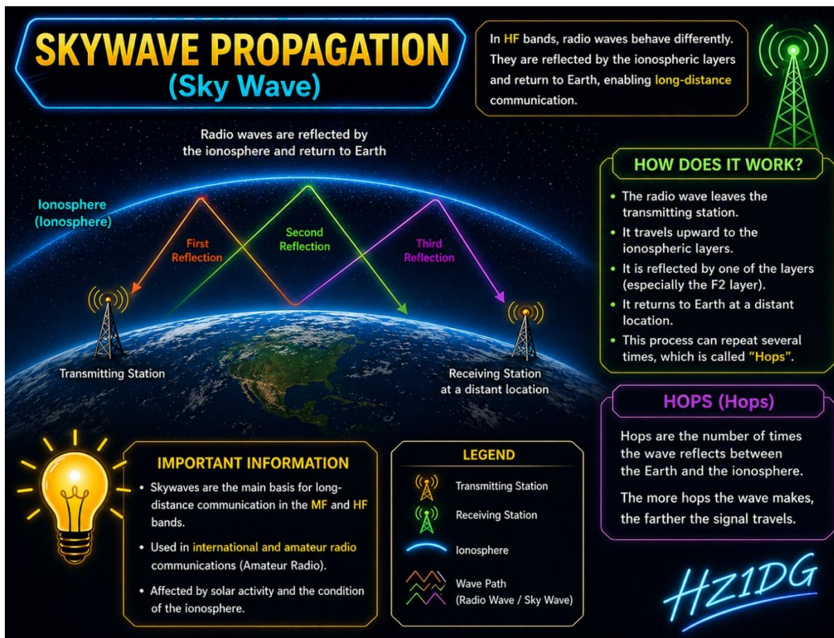
Figure (5-1): Sky wave reflection via the ionosphere
