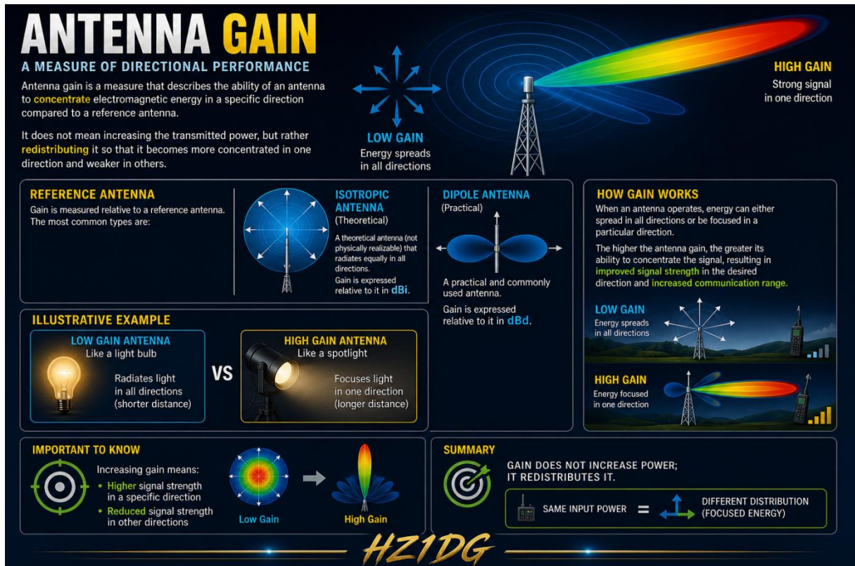
Figure (8-11): Antenna gain
