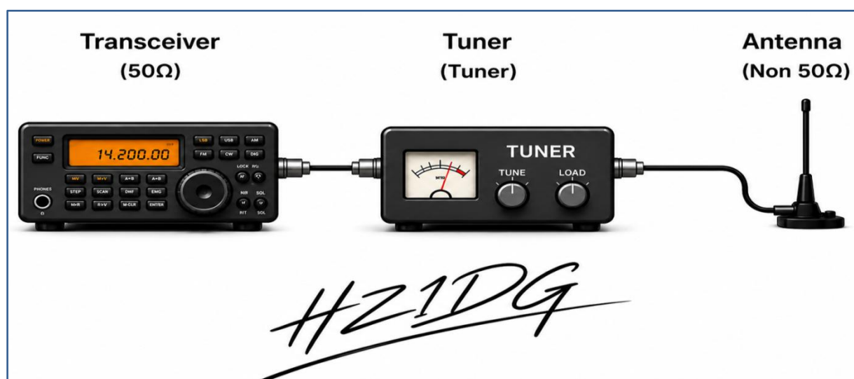
Figure (8-2): Impedance matching using an antenna tuner
