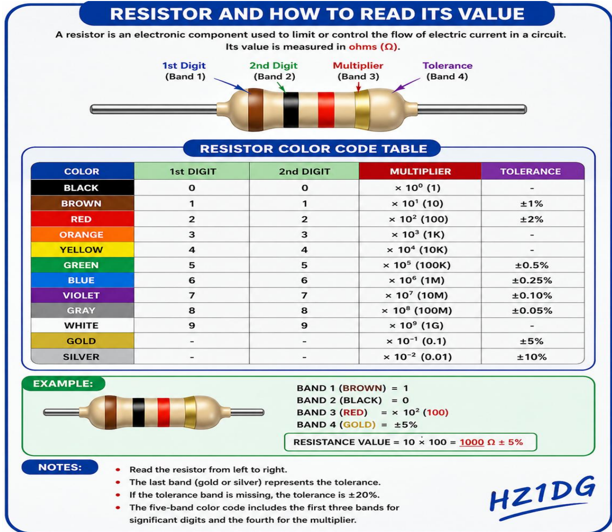
Figure (6-3): Resistor Color Code System and Value Calculation
